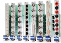
TRION-series-modules-with-high voltage-560x388
